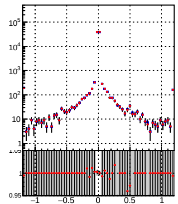
N of associated tracks (simToReco) vs dz(PV)
