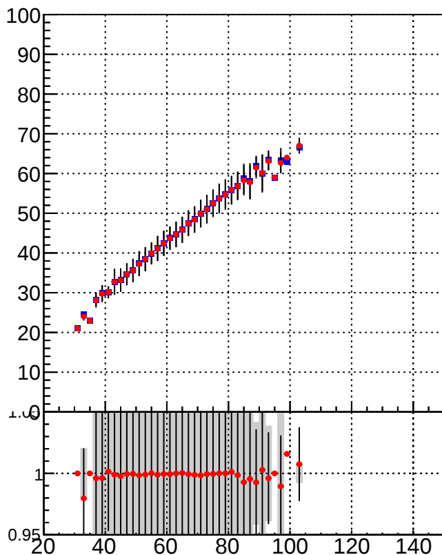
MatchedRecoVtx_vs_GenVtx
