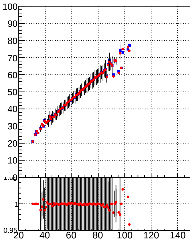
RecoVtx_vs_GenVtx
