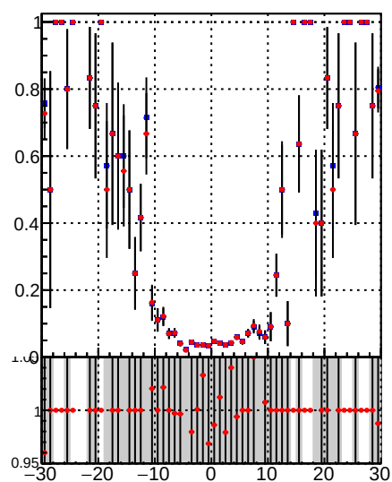
Fake rate vs d /data2/legianni/BDT-vs-DNN/real-BDT/CMSSW_13_0_0_pre4/src/runrem/DQM_TT_mkFit_ DQM_TT_mkFitRETEST3
