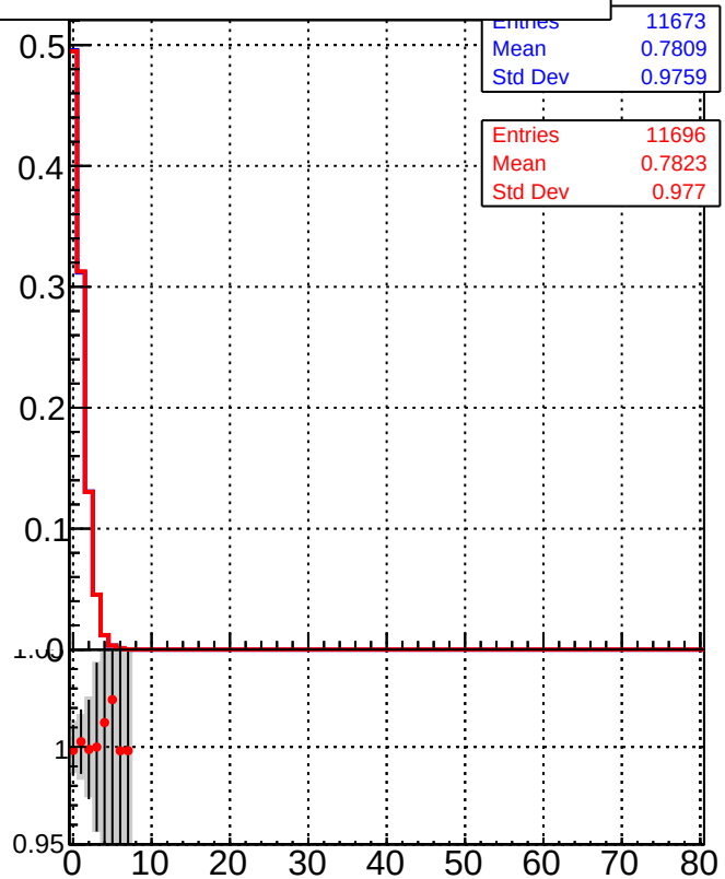
/data2/legianni/BDT-vs-DNN/real-BDT/CMSSW_13_0_0_pre4/src/runrem/DQM_TT_mkFit_ DQM_TT_mkFitRETEST3_
