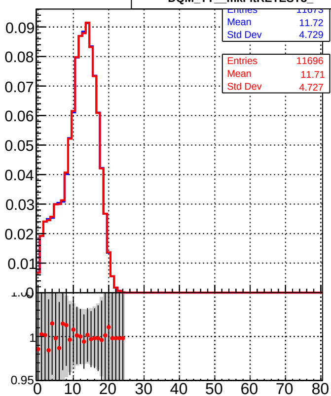
/data2/legianni/BDT-vs-DNN/real-BDT/CMSSW_13_0_0_pre4/src/runrem/DQM_TT_mkFit_ DQM_TT_mkFitRETEST3_
