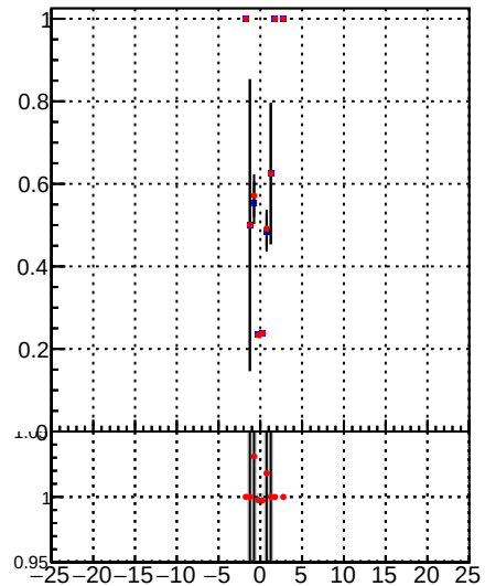
—•— /data2/legianni/BDT-vs-DNN/real-BDT/CMSSW_13_0_0_pre4/src/runrem/DQM_TT_mkFit_ —•— DQM_TT_mkFitRETEST3
