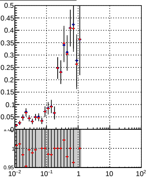
Efficiency vs vertpos — /data2/legianni/BDT-vs-DNN/real-BDT/CMSSW_13_0_0_pre4/src/runrem/DQM_TT_mkFit_ — DQM_TT_mkFitRETEST3_
