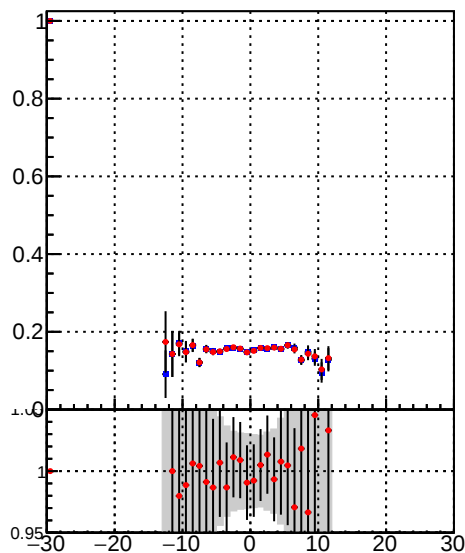
—●— /data2/legianni/BDT-vs-DNN/real-BDT/CMSSW_13_0_0_pre4/src/runrem/DQM_TT_mkFit_ —●— DQM_TT_mkFitRETEST3_
