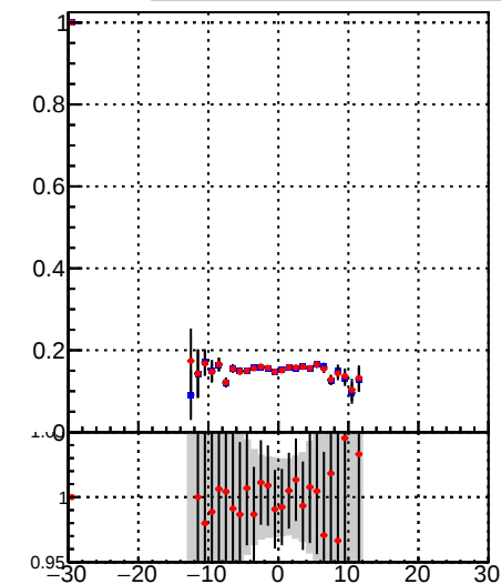
—●— /data2/legianni/BDT-vs-DNN/real-BDT/CMSSW_13_0_0_pre4/src/runrem/DQM_TT_mkFit_ —●— DQM_TT_mkFitRETEST3_
