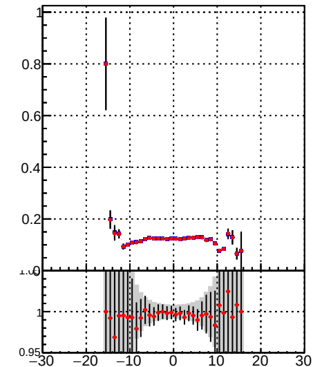
—•— /data2/legianni/BDT-vs-DNN/real-BDT/CMSSW_13_0_0_pre4/src/runrem/DQM_TT_mkFit_ —•— DQM_TT_mkFitRETEST3
