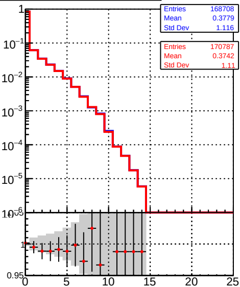
/data2/legianni/BDT-vs-DNN/real-BDT/CMSSW_13_0_0_pre4/src/runrem/DQM_TT_mkFit_ DQM_TT_mkFitRETEST3_
