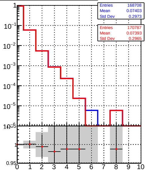
/data2/legianni/BDT-vs-DNN/real-BDT/CMSSW_13_0_0_pre4/src/runrem/DQM_TT_mkFit_ DQM_TT_mkFitRETEST3_
