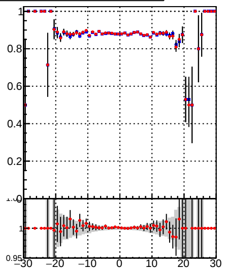
/data2/legianni/BDT-vs-DNN/real-BDT/CMSSW_13_0_0_pre4/src/runrem/DQM_TT_mkFit_ DQM_TT_mkFitRETEST3_ Pileup rate vs vertpos
