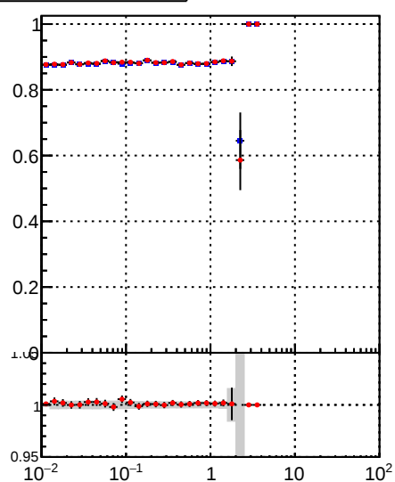
/data2/legianni/BDT-vs-DNN/real-BDT/CMSSW_13_0_0_pre4/src/runrem/DQM_TT_mkFit_ DQM_TT_mkFitRETEST3_ Pileup rate vs vertpos
