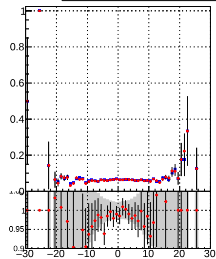
/data2/legianni/BDT-vs-DNN/real-BDT/CMSSW_13_0_0_pre4/src/runrem/DQM_TT_mkFit_ DQM_TT_mkFitRETEST3_ Fake rate vs vertpos
