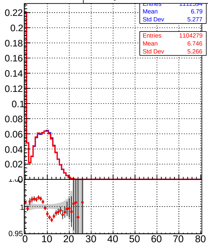
/data2/legianni/BDT-vs-DNN/real-BDT/CMSSW_13_0_0_pre4/src/runrem/DQM_TT_mkFit_ DQM_TT_mkFitRETEST3
