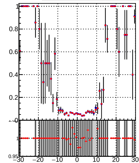
Fake rate vs v /data2/legianni/BDT-vs-DNN/real-BDT/CMSSW_13_0_0_pre4/src/runrem/DQM_TT_mkFit_ DQM_TT_mkFitRETEST3_
