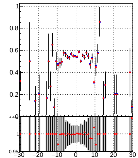
Fake rate vs v /data2/legianni/BDT-vs-DNN/real-BDT/CMSSW_13_0_0_pre4/src/runrem/DQM_TT_mkFit_ DQM_TT_mkFitRETEST3_
