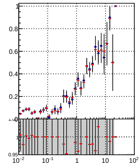
Fake rate vs v /data2/legianni/BDT-vs-DNN/real-BDT/CMSSW_13_0_0_pre4/src/runrem/DQM_TT_mkFit_ DQM_TT_mkFitRETEST3_
