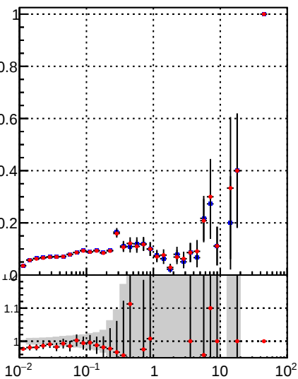
—•— /data2/legianni/BDT-vs-DNN/real-BDT/CMSSW_13_0_0_pre4/src/runrem/DQM_TT_mkFit_ —•— DQM_TT_mkFitRETEST3_ Fake rate vs v
