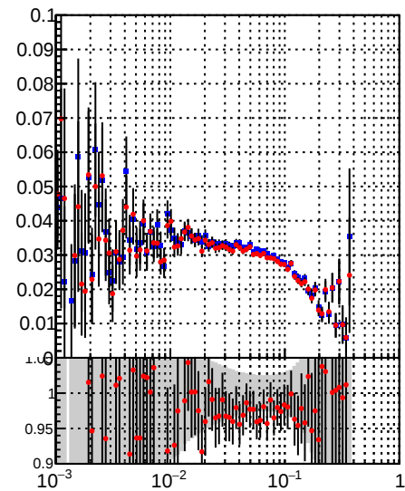
/data2/legianni/BDT-vs-DNN/real-BDT/CMSSW_13_0_0_pre4/src/runrem/DQM_TT_mkFit_ DQM_TT_mkFitRETEST3_
