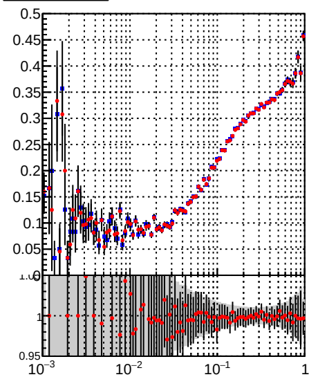
Legend: /data2/legianni/BDT-vs-DNN/real-BDT/CMSSW_13_0_0_pre4/src/runrem/DQM_TT_mkFit_ (blue squares), DQM_TT_mkFitRETEST3_ (red circles)
