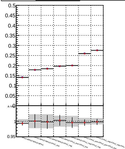
Fake rate vs. - /data2/legianni/BDT-vs-DNN/real-BDT/CMSSW_13_0_0_pre4/src/runrem/DQM_TT_mkFit_ - DQM_TT_mkFitRETEST3_
