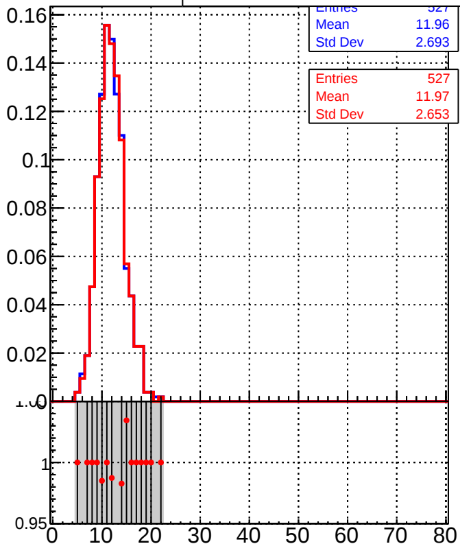
/data2/legianni/BDT-vs-DNN/real-BDT/CMSSW_13_0_0_pre4/src/runrem/DQM_TT_mkFit_ DQM_TT_mkFitRETEST3_
