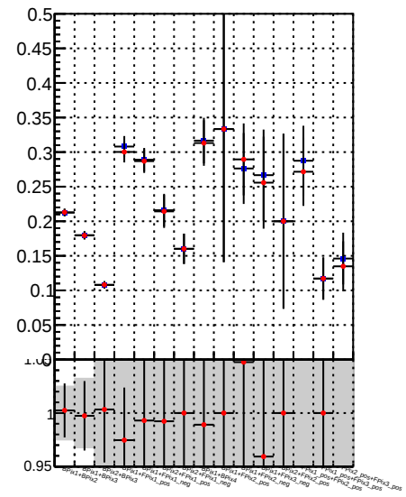
Fake rate vs. - /data2/legianni/BDT-vs-DNN/real-BDT/CMSSW_13_0_0_pre4/src/runrem/DQM_TT_mkFit_ - DQM_TT_mkFitRETEST3
