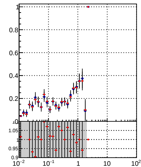
—●— /data2/legianni/BDT-vs-DNN/real-BDT/CMSSW_13_0_0_pre4/src/runrem/DQM_TT_mkFit_ —●— DQM_TT_mkFitRETEST3_ Fake rate vs vertpos
