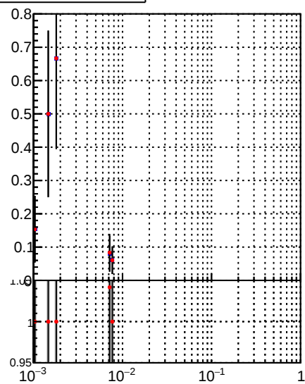
■ /data2/legianni/BDT-vs-DNN/real-BDT/CMSSW_13_0_0_pre4/src/runrem/DQM_TT_mkFit_ ● DQM_TT_mkFitRETEST3_ Duplicates Rate vs dr
