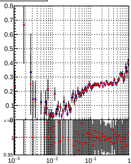
■ /data2/legianni/BDT-vs-DNN/real-BDT/CMSSW_13_0_0_pre4/src/runrem/DQM_TT_mkFit_ ● DQM_TT_mkFitRETEST3_ Pileup rate vs dr
