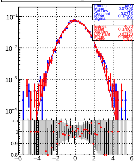
RecoPVAssoc2GenPVMatched_PulIX
