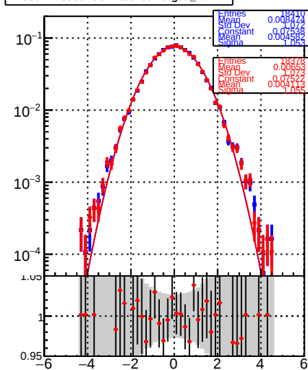
RecoAllAssoc2GenMatchedMerged_PulIX
