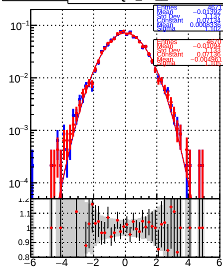
RecoPVAssoc /data2/legianni/BDT-vs-DNN/real-BDT/CMSSW_13_0_0_pre4/src/runrem/DQM_TT_mkFit_ DQM_TT_mkFitRETEST3_
