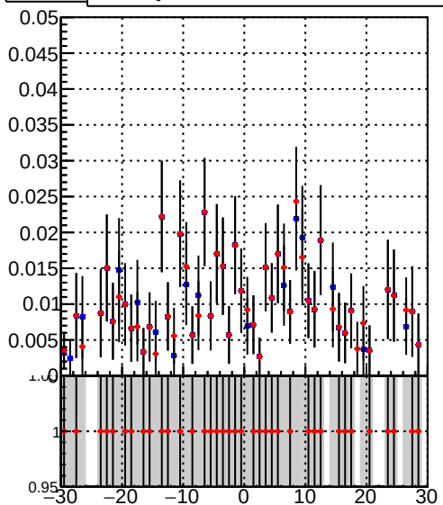
Efficiency vs vertpos - /data2/legianni/BDT-vs-DNN/real-BDT/CMSSW_13_0_0_pre4/src/runrem/DQM_TT_mkFit_ - DQM_TT_mkFitRETEST3_
