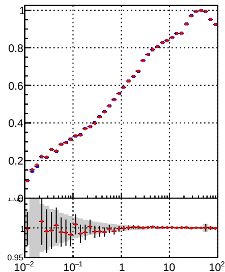
—●— /data2/legianni/BDT-vs-DNN/real-BDT/CMSSW_13_0_0_pre4/src/runrem/DQM_TT_mkFit_ —●— DQM_TT_mkFitRETEST3_
