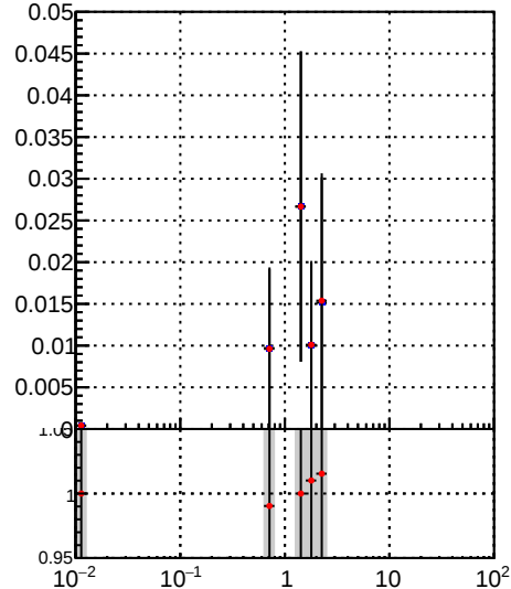
—●— /data2/legianni/BDT-vs-DNN/real-BDT/CMSSW_13_0_0_pre4/src/runrem/DQM_TT_mkFit_ —●— DQM_TT_mkFitRETEST3_
