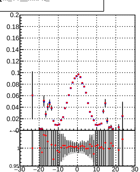
—•— /data2/legianni/BDT-vs-DNN/real-BDT/CMSSW_13_0_0_pre4/src/runrem/DQM_TT__mkFit_ —•— DQM_TT__mkFitRETEST3_
