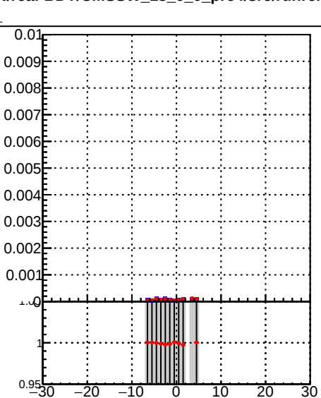
—•— /data2/legianni/BDT-vs-DNN/real-BDT/CMSSW_13_0_0_pre4/src/runrem/DQM_TT__mkFit_ —•— DQM_TT__mkFitRETEST3_
