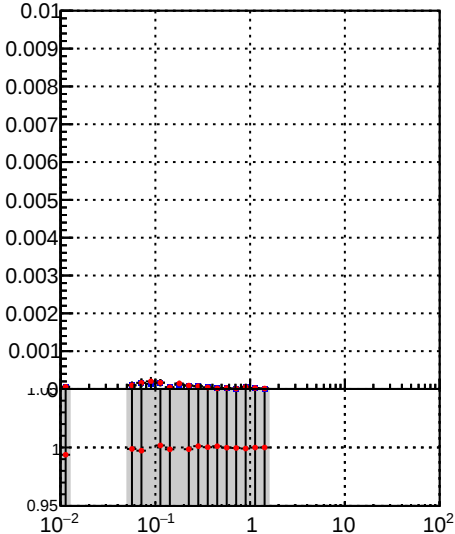
—•— /data2/legianni/BDT-vs-DNN/real-BDT/CMSSW_13_0_0_pre4/src/runrem/DQM_TT__mkFit_ —•— DQM_TT__mkFitRETEST3_
