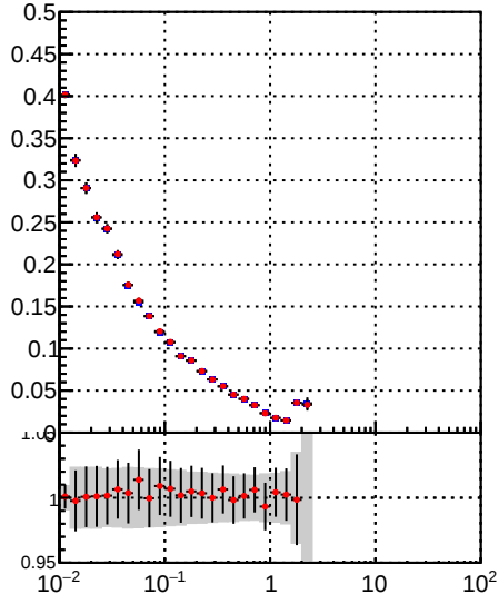
—•— /data2/legianni/BDT-vs-DNN/real-BDT/CMSSW_13_0_0_pre4/src/runrem/DQM_TT__mkFit_ —•— DQM_TT__mkFitRETEST3_
