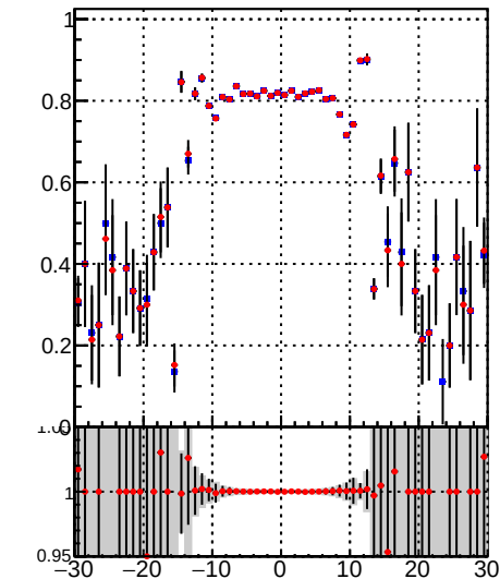
/data2/legianni/BDT-vs-DNN/real-BDT/CMSSW_13_0_0_pre4/src/runrem/DQM_TT_mkFit_ DQM_TT_mkFitRETEST3
