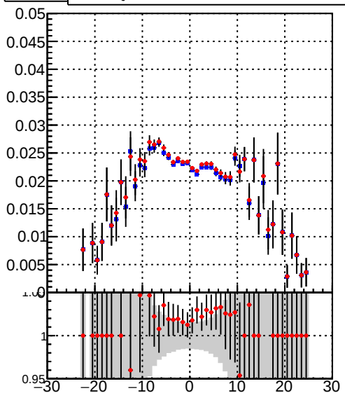
Efficiency vs vertpos - /data2/legianni/BDT-vs-DNN/real-BDT/CMSSW_13_0_0_pre4/src/runrem/DQM_TT_mkFit_ - DQM_TT_mkFitRETEST3_
