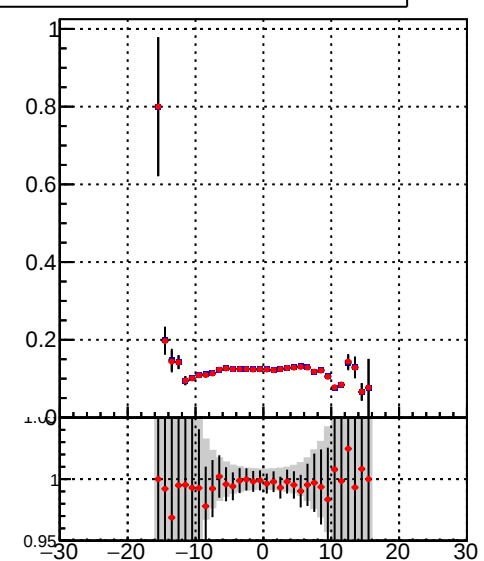
Efficiency vs vertpos - /data2/legianni/BDT-vs-DNN/real-BDT/CMSSW_13_0_0_pre4/src/runrem/DQM_TT_mkFit_ - DQM_TT_mkFitRETEST3_
