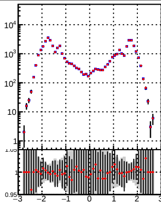
N of reco track vs \eta /data2/legianni/BDT-vs-DNN/real-BDT/CMSSW_13_0_0_pre4/src/runrem/DQM_TT_mkFit DQM_TT_mkFitRETEST3 \eta eta
