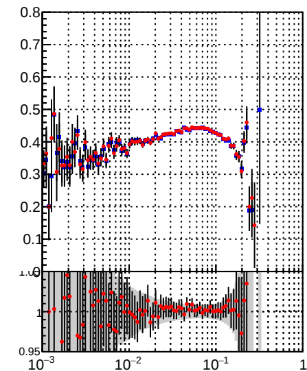
—•— /data2/legianni/BDT-vs-DNN/real-BDT/CMSSW_13_0_0_pre4/src/runrem/DQM_TT_mkFit_ —•— DQM_TT_mkFitRETEST3_
