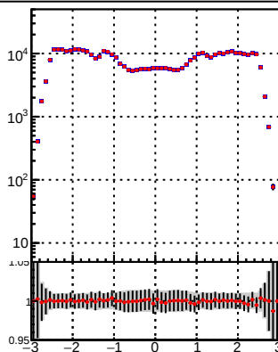
N of reco track vs \eta /data2/legianni/BDT-vs-DNN/real-BDT/CMSSW_13_0_0_pre4/src/runrem/DQM_TT_mkFit DQM_TT_mkFitRETEST3 ps eta
