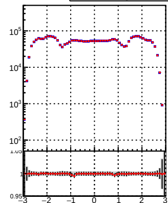
N of reco track vs \eta /data2/legianni/BDT-vs-DNN/real-BDT/CMSSW_13_0_0_pre4/src/runrem/DQM_TT_mkFit DQM_TT_mkFitRETEST3 ps eta
