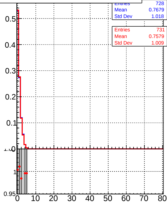
/data2/legianni/BDT-vs-DNN/real-BDT/CMSSW_13_0_0_pre4/src/runrem/DQM_TT_mkFit_ DQM_TT_mkFitRETEST3_
