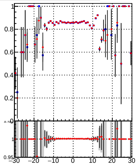
—●— /data2/legianni/BDT-vs-DNN/real-BDT/CMSSW_13_0_0_pre4/src/runrem/DQM_TT_mkFit_ —●— DQM_TT_mkFitRETEST3_ Pileup rate vs
