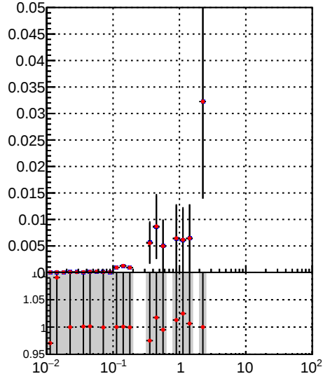
—●— /data2/legianni/BDT-vs-DNN/real-BDT/CMSSW_13_0_0_pre4/src/runrem/DQM_TT_mkFit_ —●— DQM_TT_mkFitRETEST3_ Duplicates Rate vs
