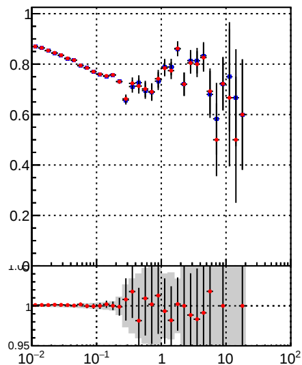
—●— /data2/legianni/BDT-vs-DNN/real-BDT/CMSSW_13_0_0_pre4/src/runrem/DQM_TT_mkFit_ —●— DQM_TT_mkFitRETEST3_ Pileup rate vs
