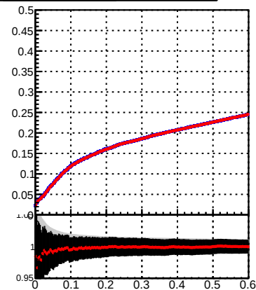
Fake rate Legend: █ /data2/legianni/BDT-vs-DNN/real-BDT/CMSSW_13_0_0_pre4/src/runrem/DQM_TT_mkFit_ █ DQM_TT_mkFitRETEST3_
