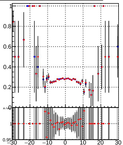
—•— /data2/legianni/BDT-vs-DNN/real-BDT/CMSSW_13_0_0_pre4/src/runrem/DQM_TT_mkFit_ —•— DQM_TT_mkFitRETEST3_
