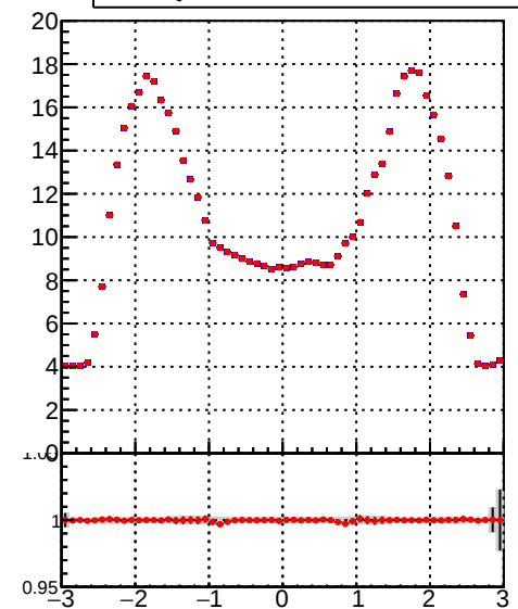
/data2/legianni/BDT-vs-DNN/real-BDT/CMSSW_13_0_0_pre4/src/runrem/DQM_TT__mkFit_ DQM_TT__mkFitRETEST3_
