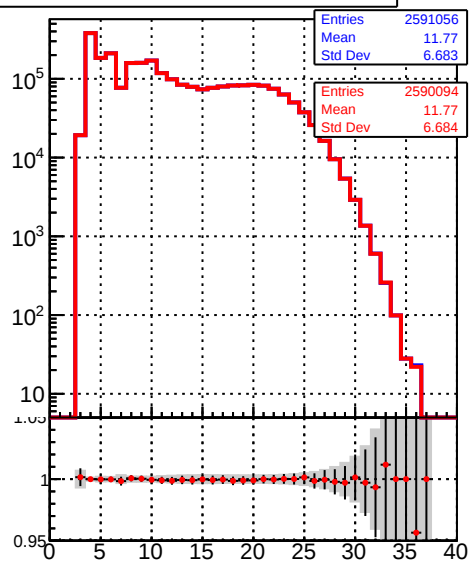
/data2/legianni/BDT-vs-DNN/real-BDT/CMSSW_13_0_0_pre4/src/runrem/DQM_TT__mkFit_ DQM_TT__mkFitRETEST3_
