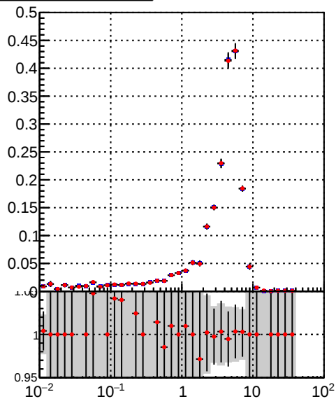
—•— /data2/legianni/BDT-vs-DNN/real-BDT/CMSSW_13_0_0_pre4/src/runrem/DQM_TT_mkFit_ —•— DQM_TT_mkFitRETEST3_
