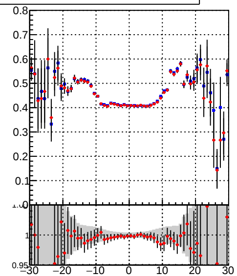
—•— /data2/legianni/BDT-vs-DNN/real-BDT/CMSSW_13_0_0_pre4/src/runrem/DQM_TT_mkFit_ —•— DQM_TT_mkFitRETEST3_
