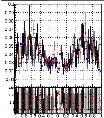
Efficiency vs D_{xy} (PV) - \bullet /data2/legianni/BDT-vs-DNN/real-BDT/CMSSW_13_0_0_pre4/src/runrem/DQM_TT_mkFit_ - \bullet DQM_TT_mkFitRETEST2_
