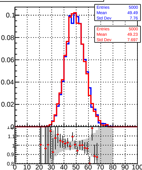
ReconstructedAllAssoc2Gen_NumVertices
