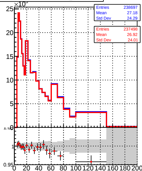
ReconstructedAllAssoc2Gen_NumTracks
