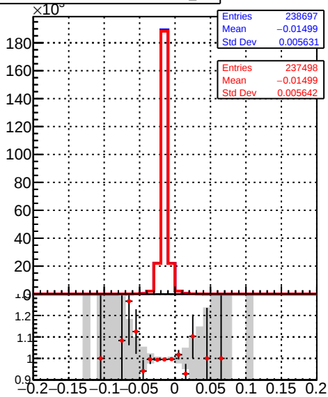
ReconstructedAllAssoc2Gen_Y
