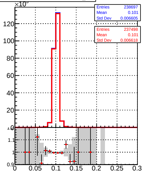
ReconstructedAllAssoc2Gen_X
