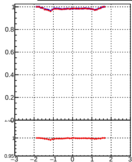
—•— /data2/legianni/BDT-vs-DNN/real-BDT/CMSSW_13_0_0_pre4/src/runrem/DQM_TT_mkFit_ —•— DQM_TT_mkFitRETEST2_
