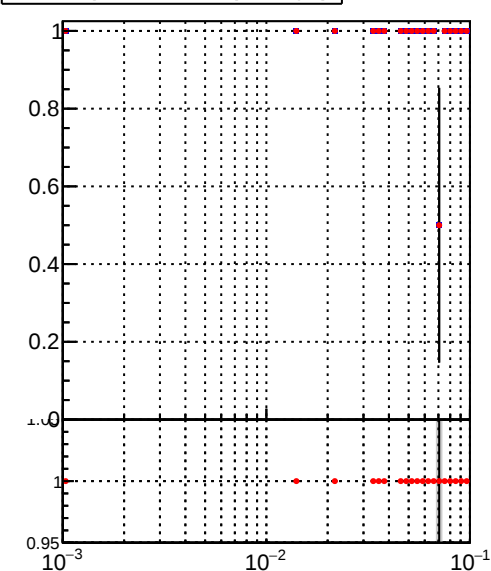
fake+duplicates vs \Delta R(\text{track}, \text{jet})
