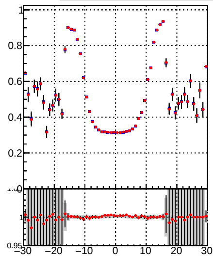
—•— /data2/legianni/BDT-vs-DNN/real-BDT/CMSSW_13_0_0_pre4/src/runrem/DQM_TT_mkFit_ —•— DQM_TT_mkFitRETEST2_
