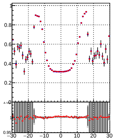
/data2/legianni/BDT-vs-DNN/real-BDT/CMSSW_13_0_0_pre4/src/runrem/DQM_TT_mkFit_ DQM_TT_mkFitRETEST2
