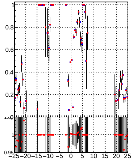
/data2/legianni/BDT-vs-DNN/real-BDT/CMSSW_13_0_0_pre4/src/runrem/DQM_TT_mkFit_ DQM_TT_mkFitRETEST2
