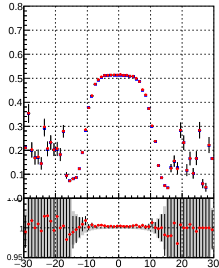
/data2/legianni/BDT-vs-DNN/real-BDT/CMSSW_13_0_0_pre4/src/runrem/DQM_TT_mkFit_ DQM_TT_mkFitRETEST2
