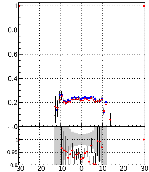
—•— /data2/legianni/BDT-vs-DNN/real-BDT/CMSSW_13_0_0_pre4/src/runrem/DQM_TT_mkFit_ —•— DQM_TT_mkFitRETEST2_
