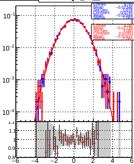
RecoPVAssoc /data2/legianni/BDT-vs-DNN/real-BDT/CMSSW_13_0_0_pre4/src/runrem/DQM_TT_mkFit_ DQM_TT_mkFitRETEST2_
