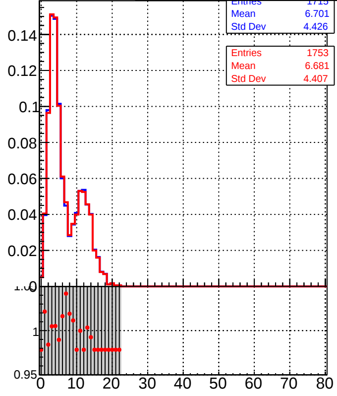
/data2/legianni/BDT-vs-DNN/real-BDT/CMSSW_13_0_0_pre4/src/runrem/DQM_TT_mkFit_ DQM_TT_mkFitRETEST2_
