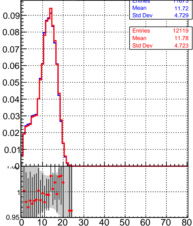
■ /data2/legianni/BDT-vs-DNN/real-BDT/CMSSW_13_0_0_pre4/src/runrem/DQM_TT_mkFit_ ● DQM_TT_mkFitRETEST2_
