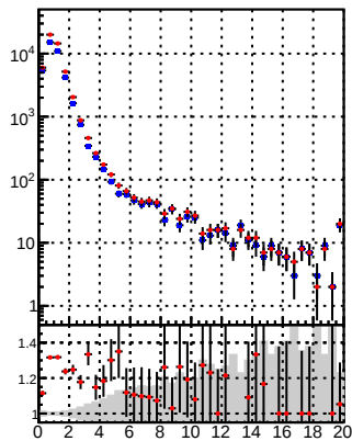
N of reco track vs. \chi^2 /data2/legianni/BDT-vs-DNN/real-BDT/CMSSW_13_0_0_pre4/src/runrem/DQM_TT_mkFit DQM_TT_mkFitRETEST2
