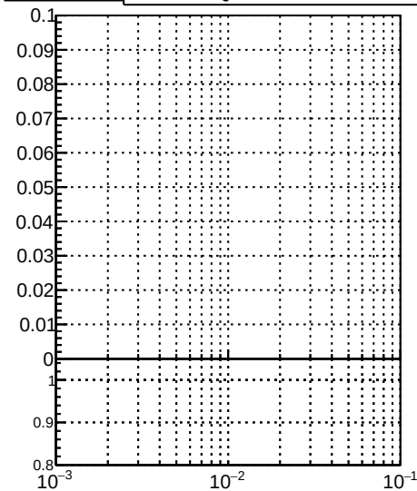
/data2/legianni/BDT-vs-DNN/real-BDT/CMSSW_13_0_0_pre4/src/runrem/DQM_TT_mkFit_ DQM_TT_mkFitRETEST2_ Fake rate vs
