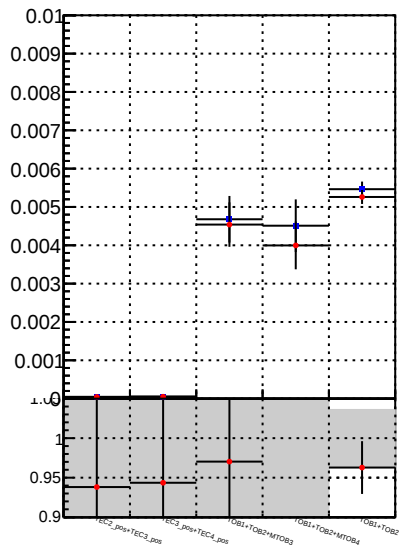
—●— /data2/legianni/BDT-vs-DNN/real-BDT/CMSSW_13_0_0_pre4/src/runrem/DQM_TT_mkFit_ —●— DQM_TT_mkFitRETEST2
