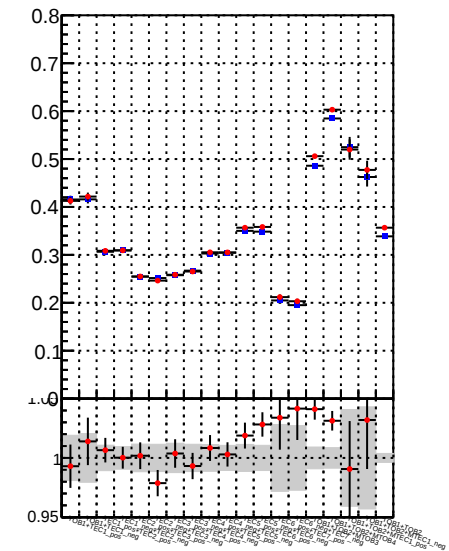
—●— /data2/legianni/BDT-vs-DNN/real-BDT/CMSSW_13_0_0_pre4/src/runrem/DQM_TT_mkFit_ —●— DQM_TT_mkFitRETEST2
